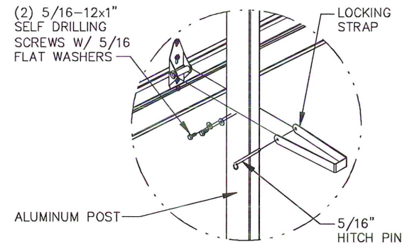
DETAIL F
