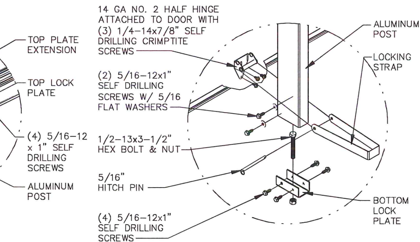
DETAIL G
